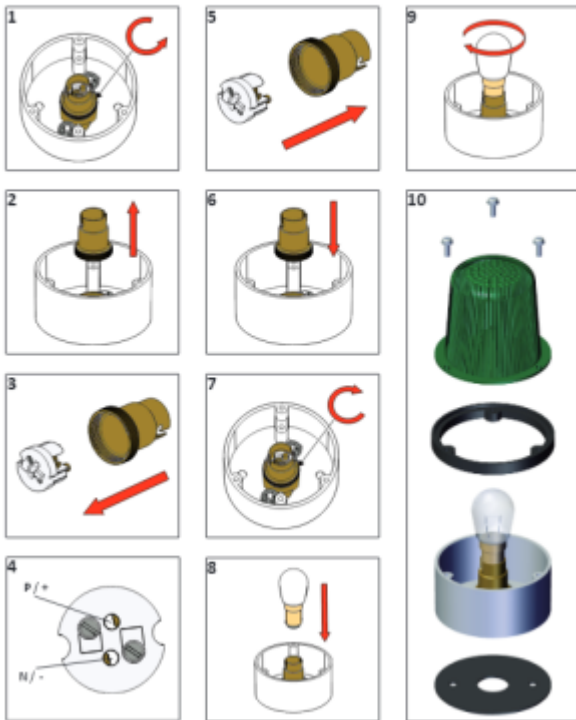
SBD/B15d Static Filament Beacon
